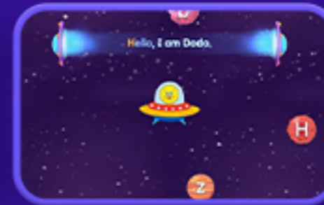
Sentence Activity
